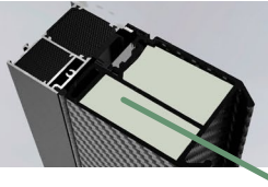
HYBRID OF ALUMINUM FRAME AND CARBON STRUCTURED FIBER GLASS COMPOSITE
